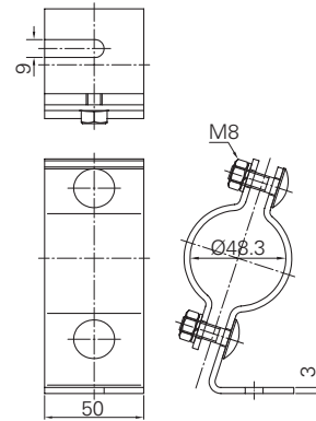
Ceiling bracket D92
